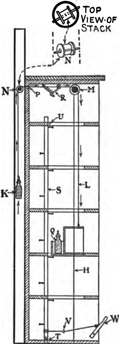
FIG. 97. — Section through Elevator Shaft.
